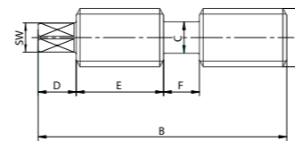
Adjusting spindle
