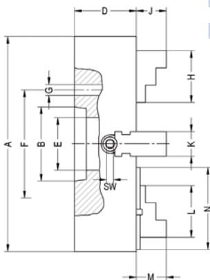
DIN 55026 mounting from front
