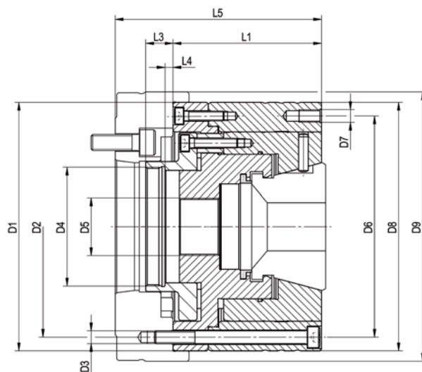
CAPTIS-AF collet chuck - axially fixed collet chuck, no axial tension against internal workpiece stop
