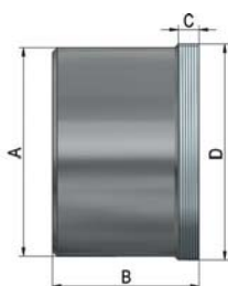
C 15 Connecting piece for collet chuck KZF
